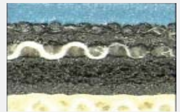
Vulcan Editor 10
